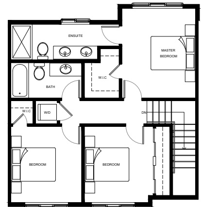
THIRD FLOOR
