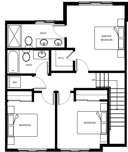
THIRD FLOOR
